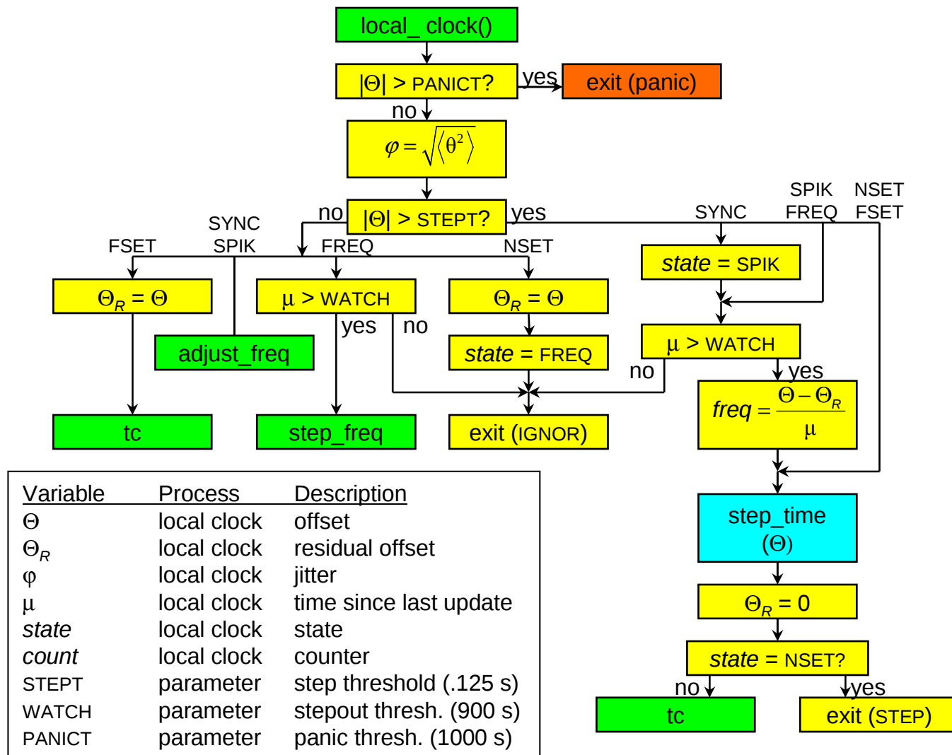
local_clock() Function
